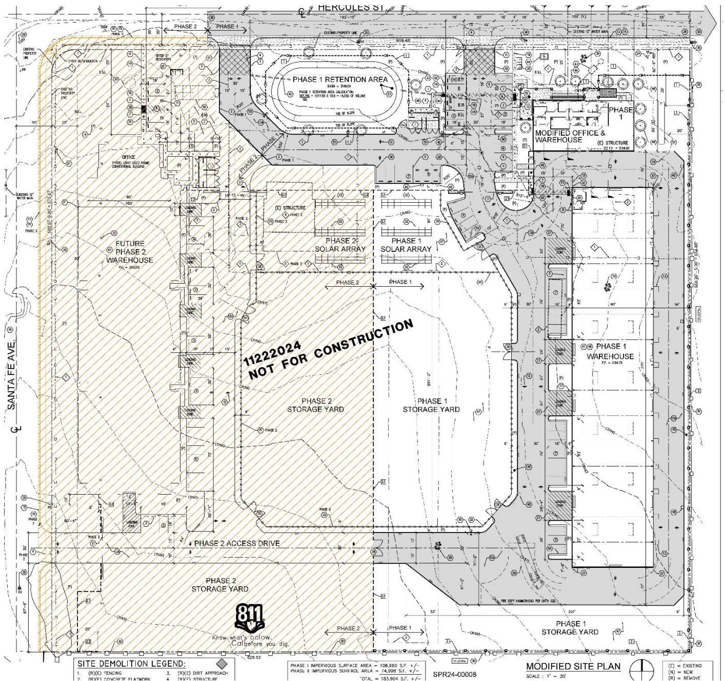
Figure 2 – Site Plan Schematic
